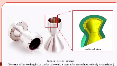
Sub-scale rocket nozzle (Because of the cooling holes on the side wall, it cannot be manufactured only by machine.)
